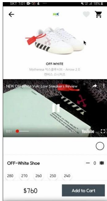
item detail
