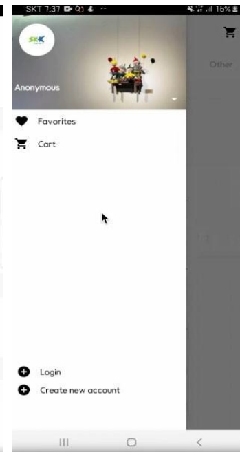
profile
