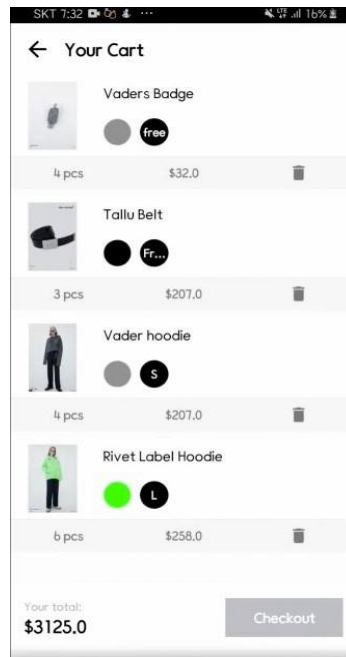
cart
